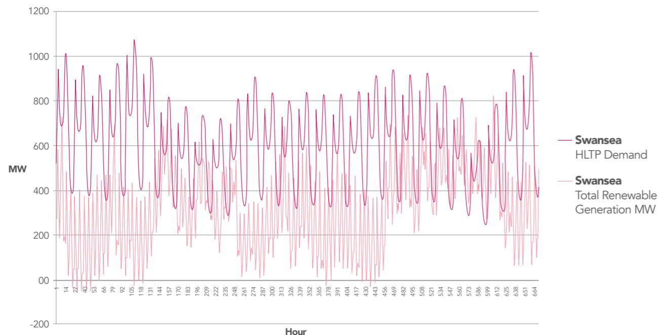
Figure 7. Swansea heat, light, power & transport supply & demand profiles, December 2030
