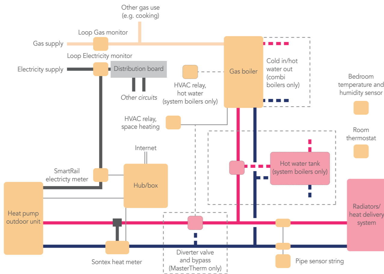
Figure 16. Meter schematic
