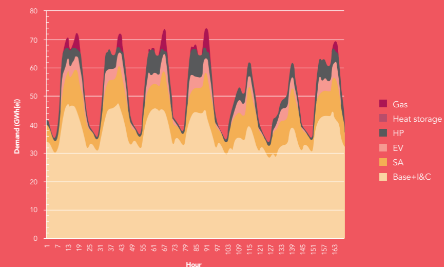
Figure 8. Electricity demand and equivalent heat pump gas demand.
