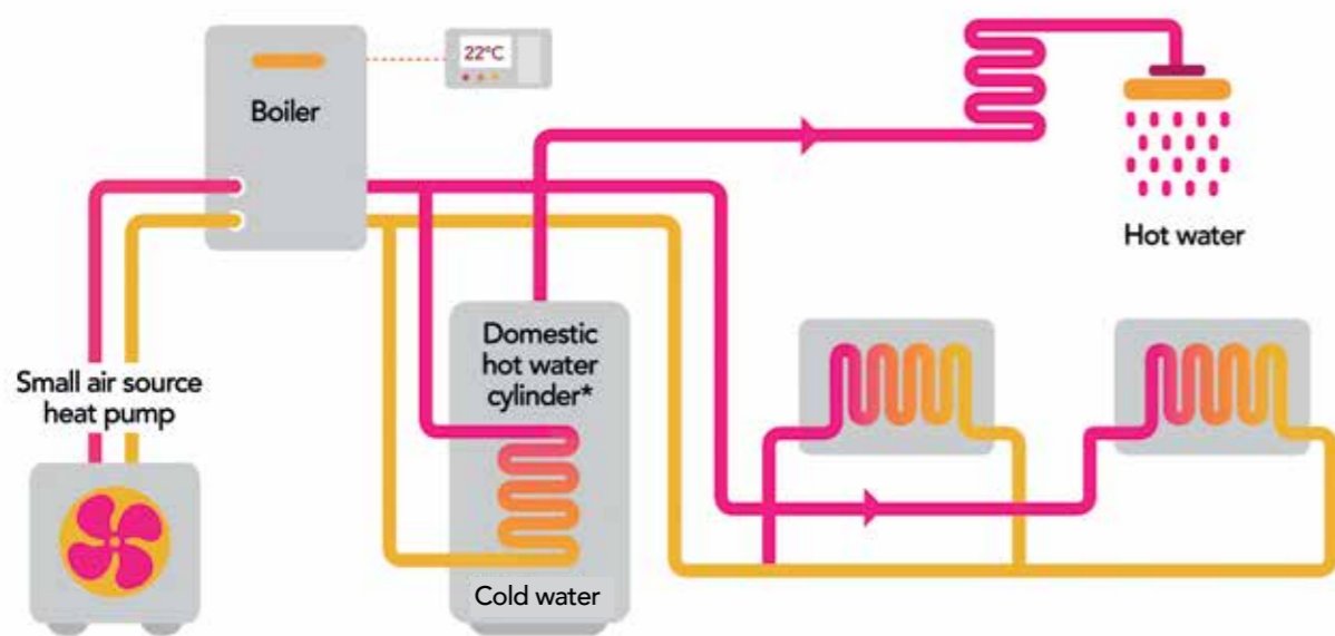
Figure 1. The hybrid system * Optional
