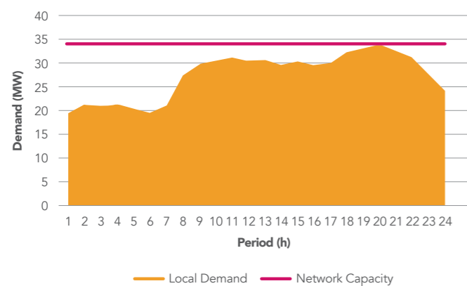
Figure 11. Local electricity demand at primary substation level and secured network capacity in a typical winter day.
