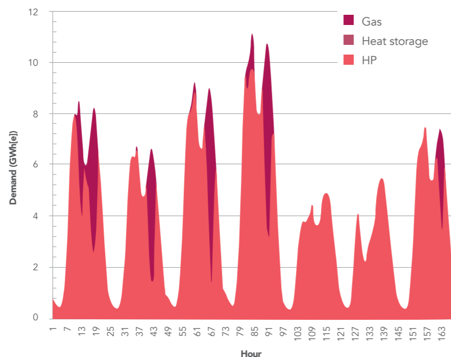
Figure 9. Hybrid heating system switching based upon electricity network capacity constraints
