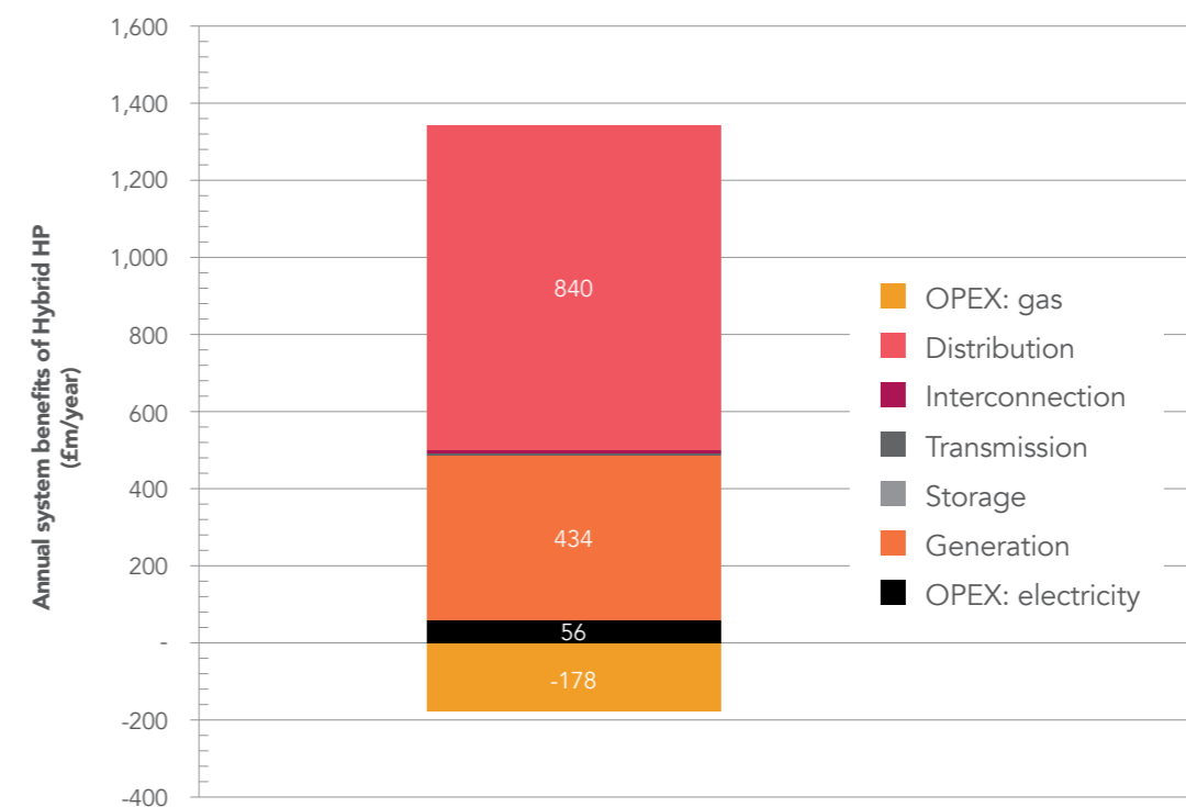
Figure 10. Imperial College modelled system-level benefits of hybrid heating systems
