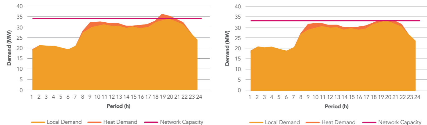
Figure 12. Local and electrified heat demand at the distribution network (a) without and (b) with network support service.
